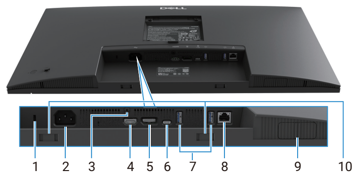
Figure 6. Bottom view without monitor stand
