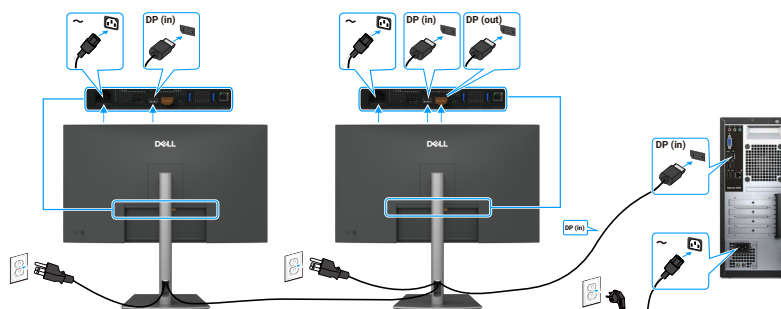
Figure 30. Connecting the monitor for DP Multi-Stream Transport (MST) function
